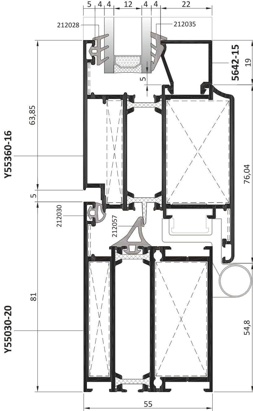
KATLANIR KAPI FOLDING DOOR
