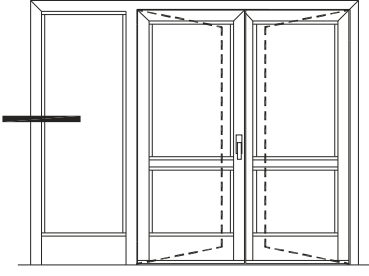
DIŐA AÇILIR HEMYÖZ KAPI OUTWARD OPENING FLUSH DOOR
