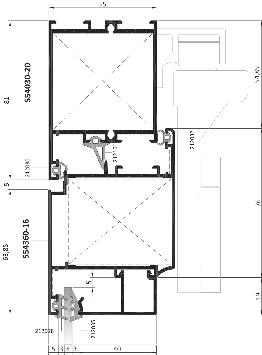
KATLANIR KAPI FOLDING DOOR
