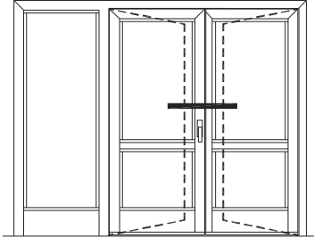
DIŐA AÇILIR HEMYÜZ KAPI OUTWARD OPENING FLUSH DOOR
