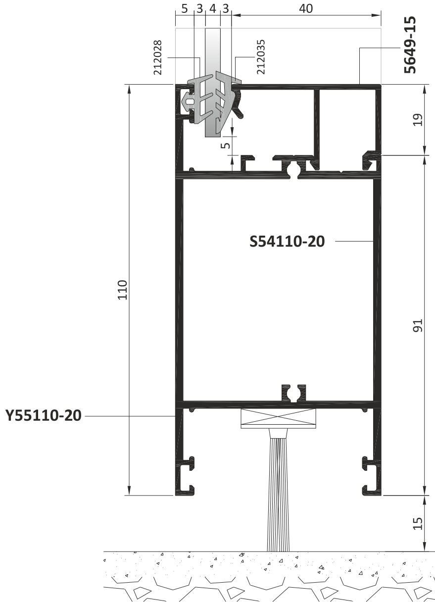
DIŐA AÇILIR HEMYÜZ KAPI OUTWARD OPENING FLUSH DOOR
