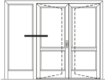
DIŐA AÇILIR BİNİLİ KAPI OUTWARD OPENING DOOR WITH STEP HINGE
