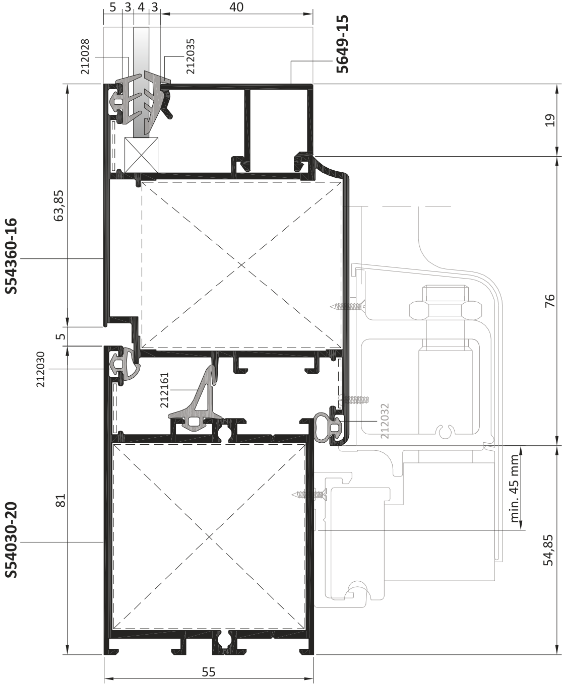
KATLANIR KAPI FOLDING DOOR
