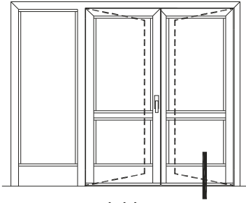
DIŐA AÇILIR BİNİLİ KAPI OUTWARD OPENING DOOR WITH STEP HINGE
