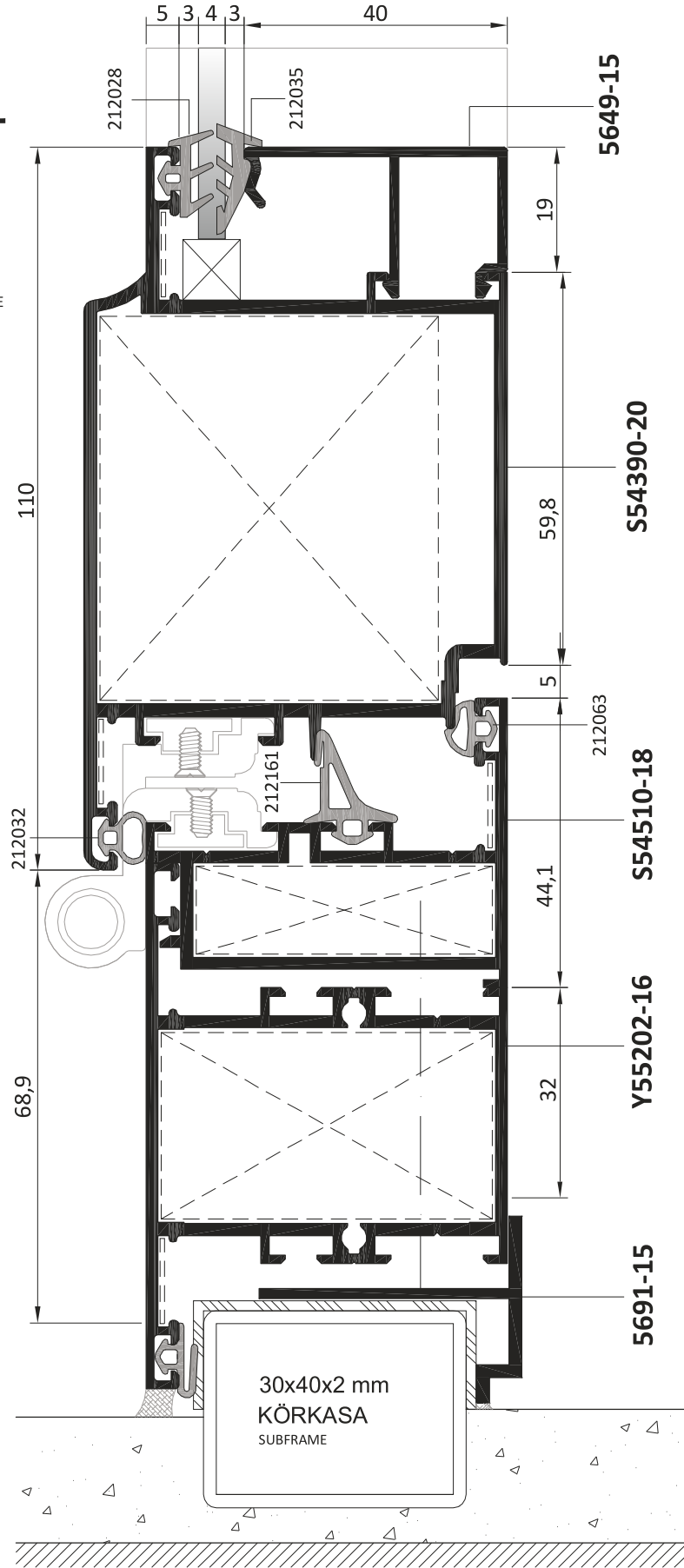
DIŐA AÇILIR BİNİLİ KAPI OUTWARD OPENING DOOR WITH STEP HINGE
