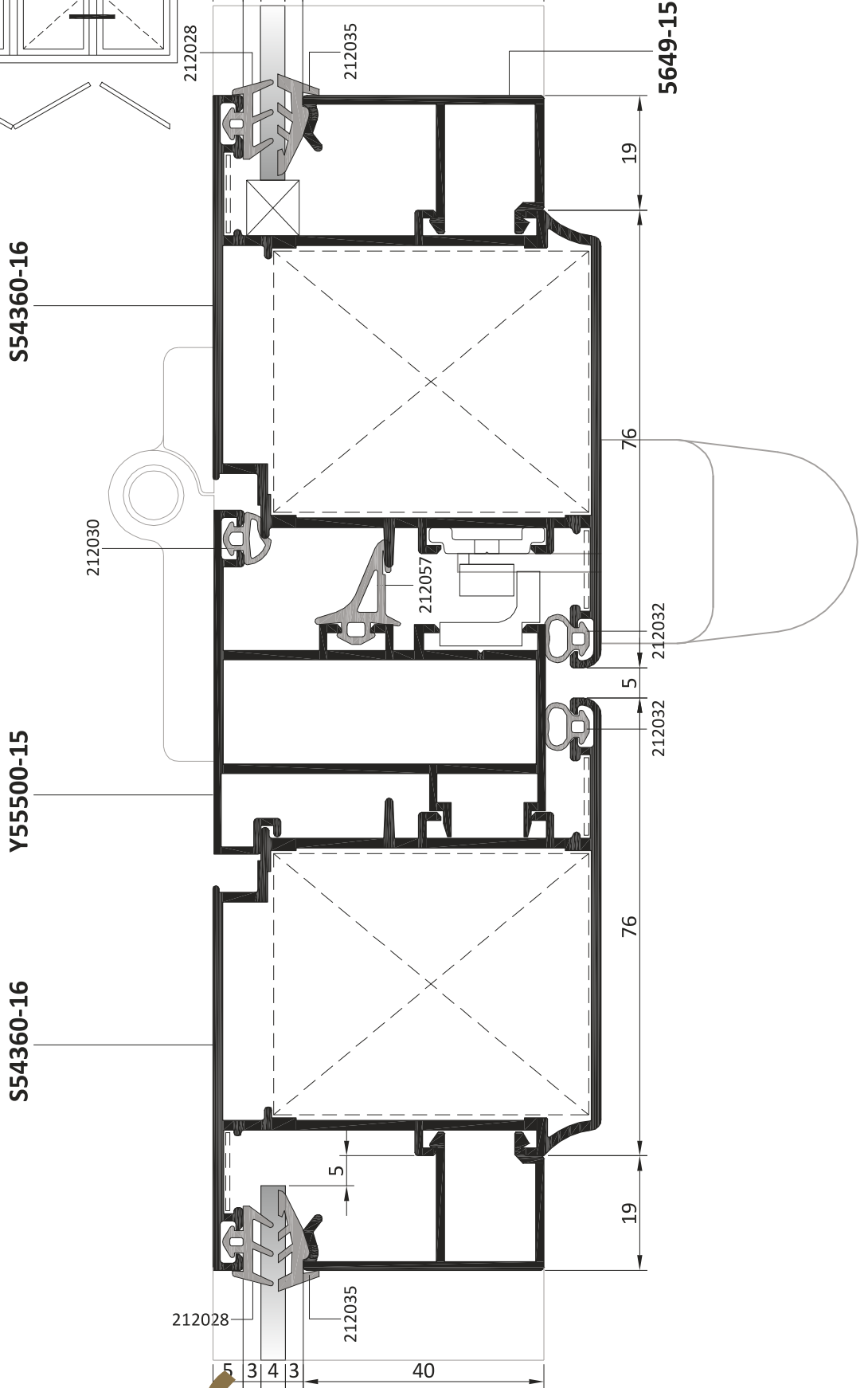
KATLANIR KAPI FOLDING DOOR
